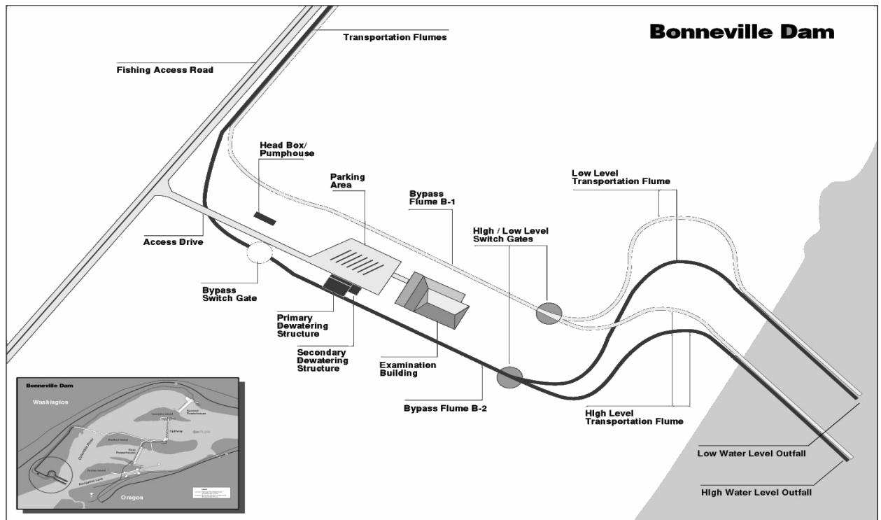
Figure B-8. Hamilton Island Juvenile Monitoring Facility, Bonneville Dam.
