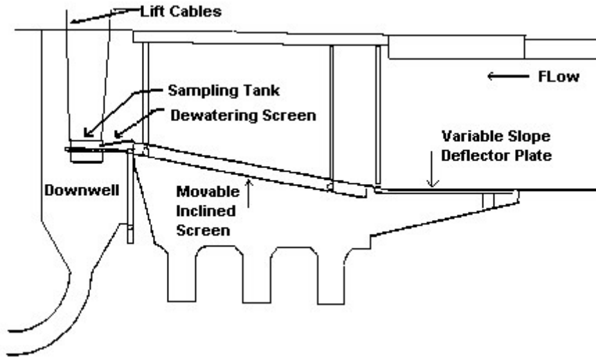
Figure C-8. PH1 inclined screen sampling system, 1986-2001.
